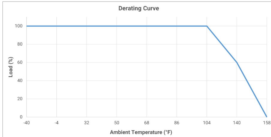
Derating Curve
